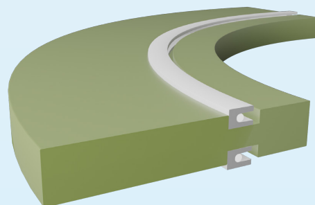
Stainless Steel Core (SSC) Spring-Energized Seal 385°F
